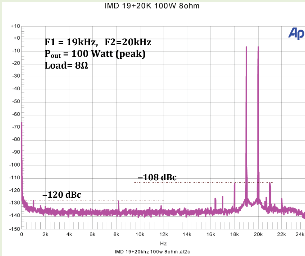
Fig. 5b DC-24 kHz Intermodulation Distortion spectrum. Freq=19kHz+20kHz. Load=8Ω. Output power=100W peak.
