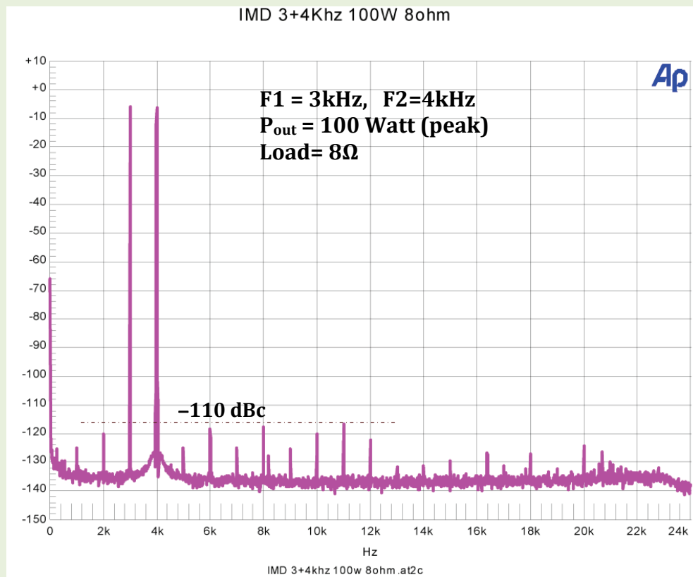
Fig. 5a: DC-24 kHz Intermodulation Distortion spectrum. Freq=3kHz+4kHz. Load=8Ω. Output power=100W peak.
