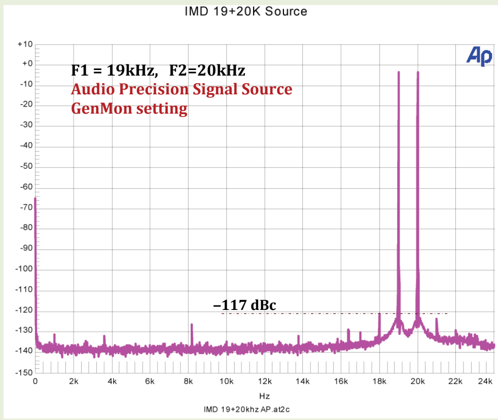
Fig. 5c: DC-24 kHz IMD Distortion spectrum. Freq=19kHz+20kHz. Signal Source with AP test equipment in GenMon setting.
