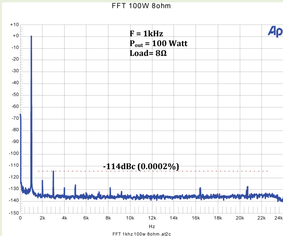
Fig. 3c: DC-24 kHz harmonic distortion spectrum. Freq=1kHz. Load=8Ω. Output power=100W.
