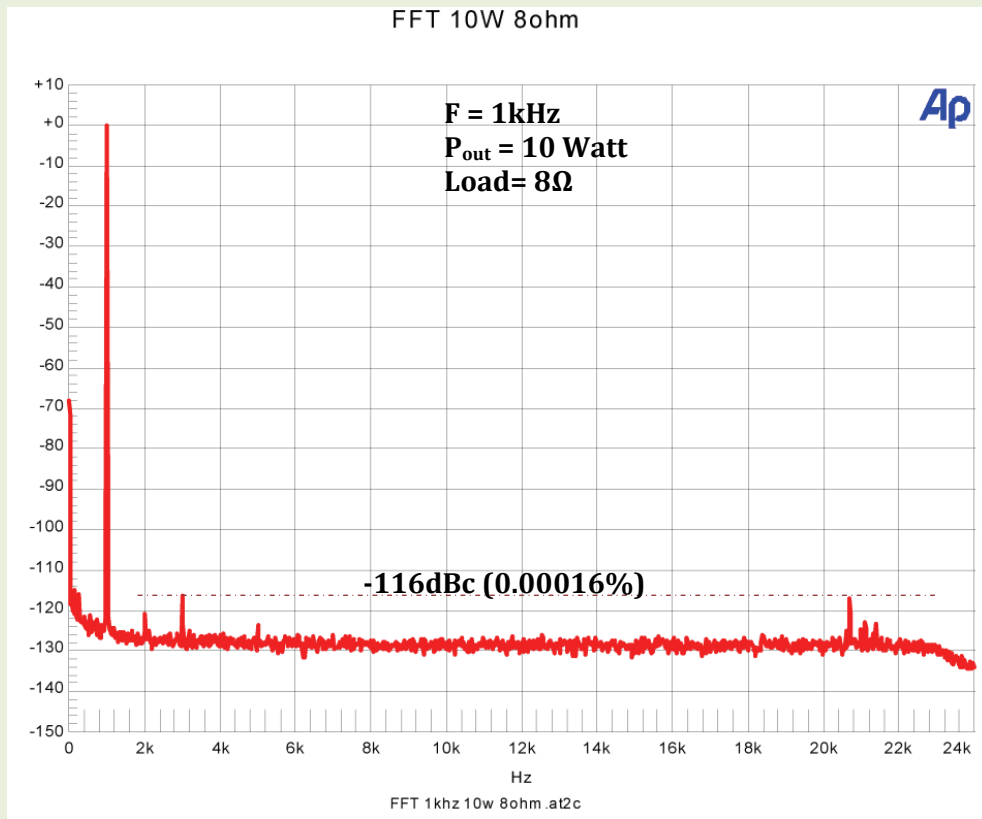
Fig. 3b: DC-24 kHz harmonic distortion spectrum. Freq=1kHz. Load=8Ω. Output power=10W.
