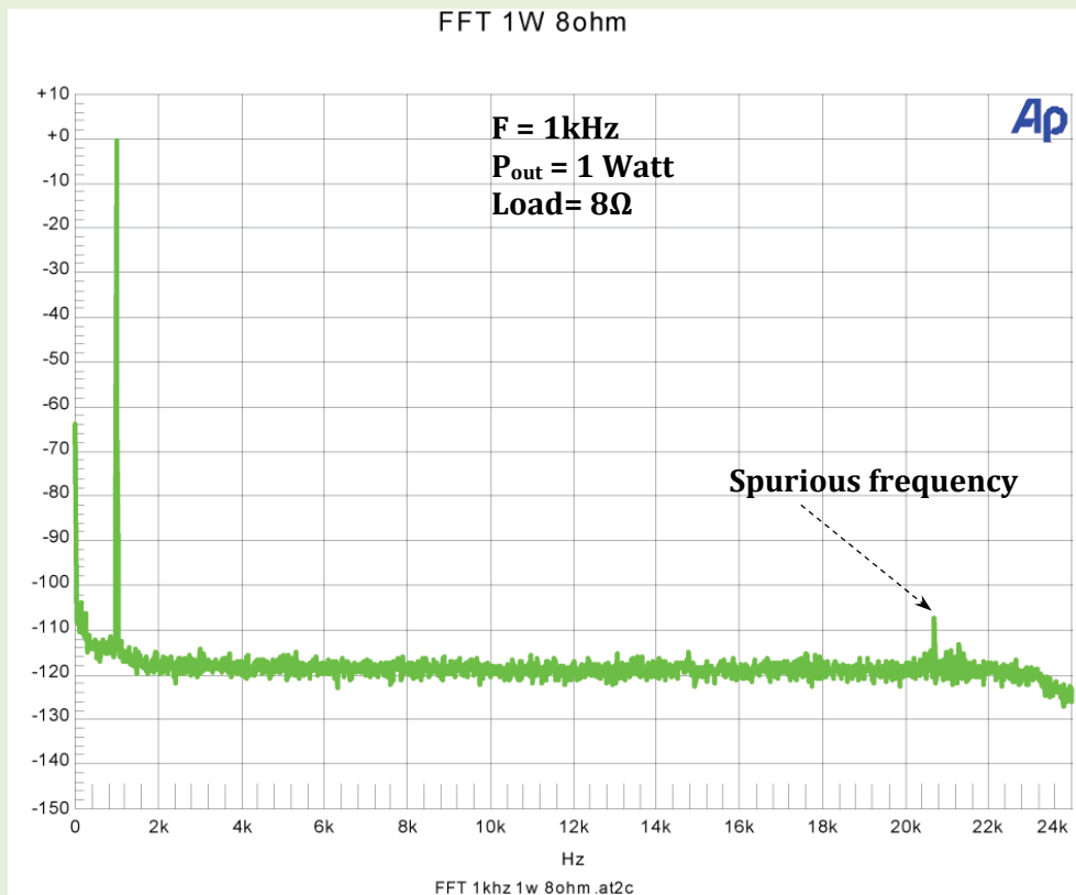
Fig. 3a: DC-24 kHz harmonic distortion spectrum. Freq=1kHz. Load= 8\Omega . Output power=1W.
