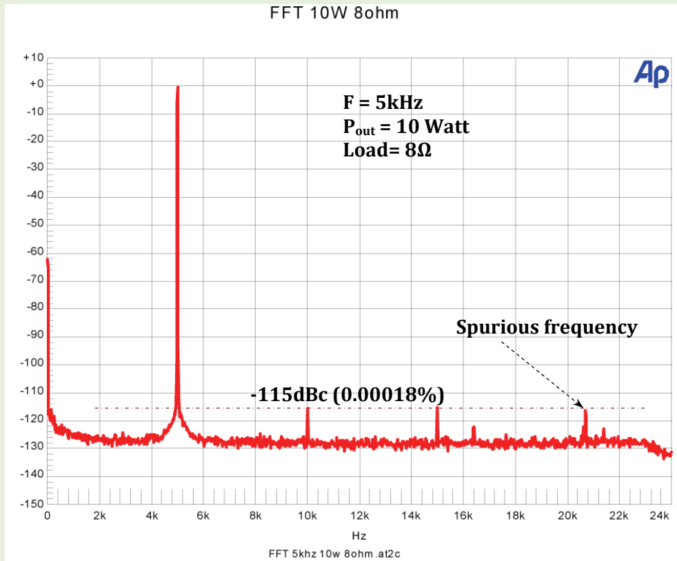
Fig. 4b: DC-24 kHz Harmonic Distortion spectrum. Freq=5kHz. Load=8Ω. Output power=10W.
