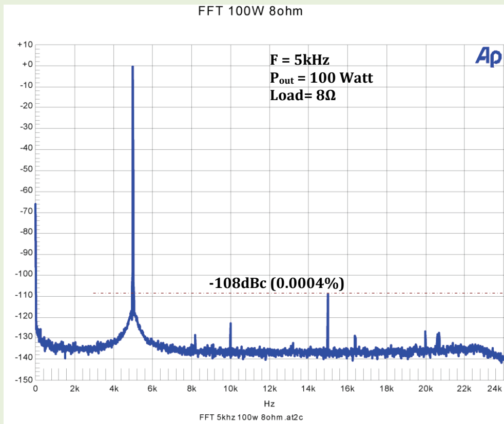
Fig. 4c: DC-24 kHz harmonic distortion spectrum. Freq=5kHz. Load=8Ω. Output power=100W.
