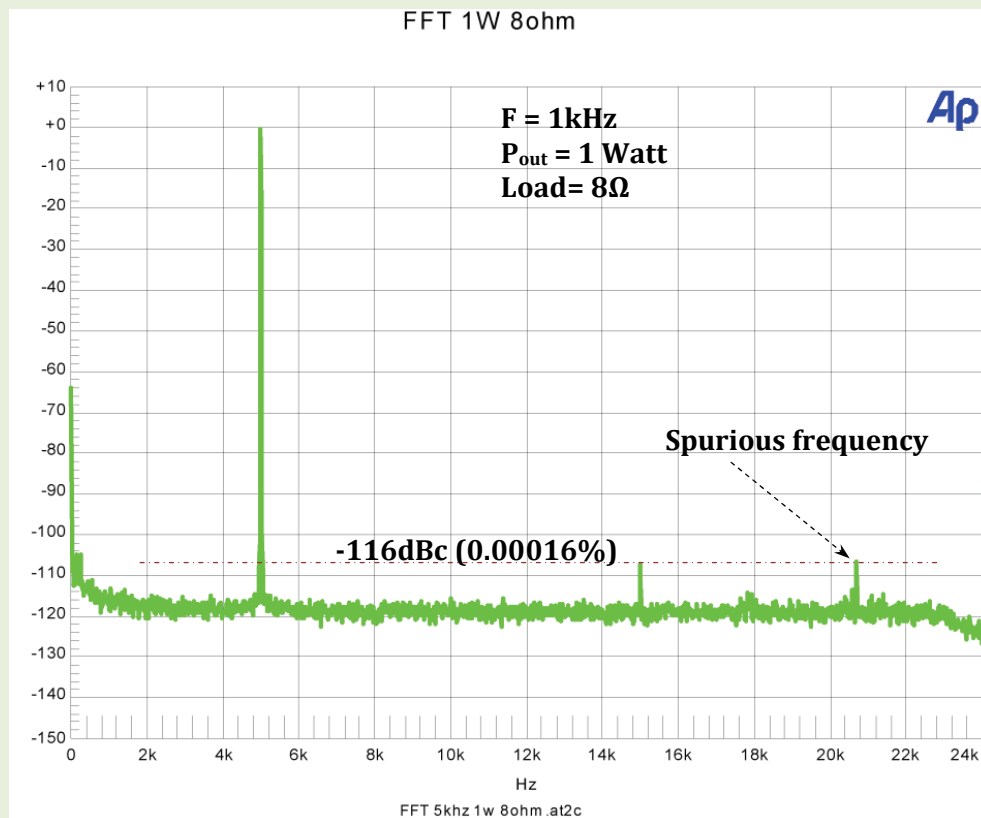
Fig. 4a: DC-24 kHz Harmonic Distortion spectrum. Freq=5kHz. Load=8Ω. Output power=1W.
