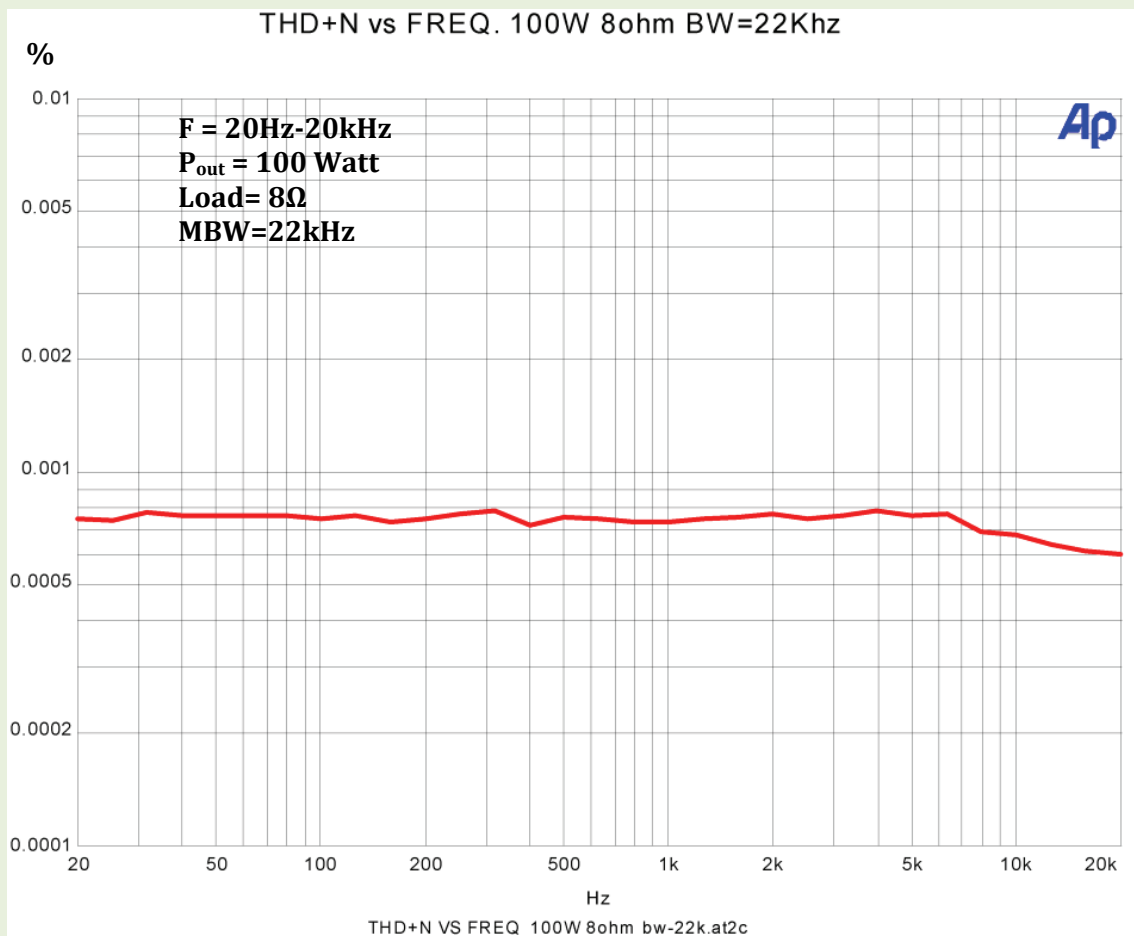
Fig. 2a: THD+N (%) versus frequency. Freq=20Hz-20kHz. Load=8Ω. Output power=100W. Measurement bandwidth (MBW)=22kHz
