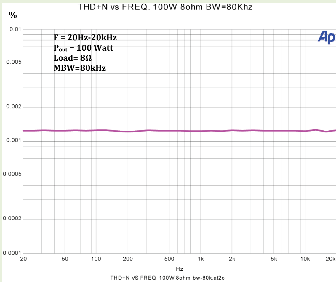
Fig. 2b: THD+N (%) versus frequency. Freq=20Hz-20kHz. Load=8Ω. Output power=100W. Measurement bandwidth (MBW)=80kHz
