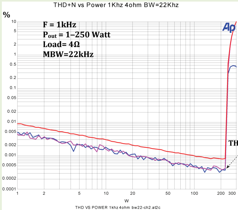
Fig. 1b: THD+N (%) versus power. Frequency=1kHz, Load=4Ω. Measurement bandwidth (MBW)=22kHz
