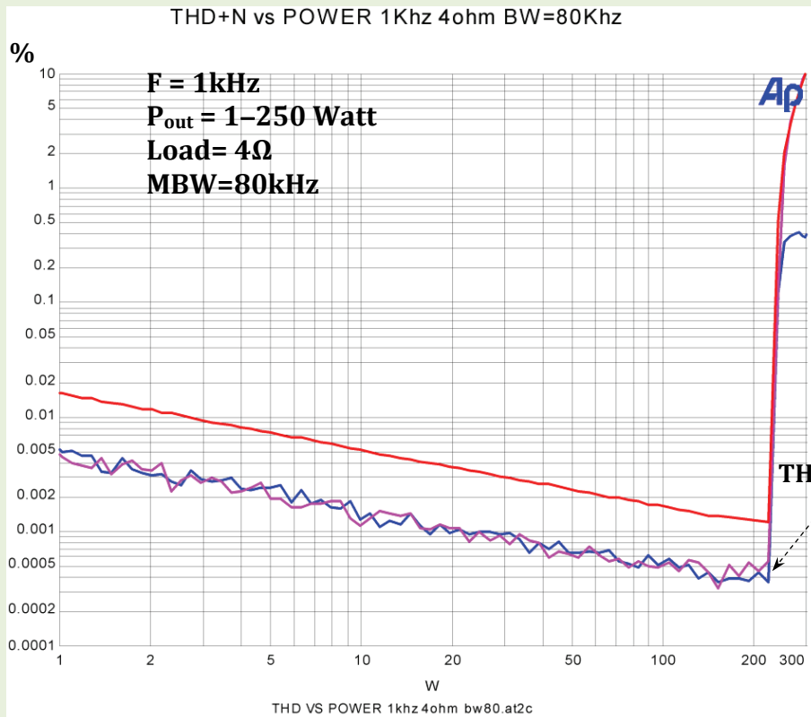
Fig. 1c: THD+N (%) versus power. Frequency=1kHz, Load=4Ω. Measurement bandwidth (MBW)=80kHz
