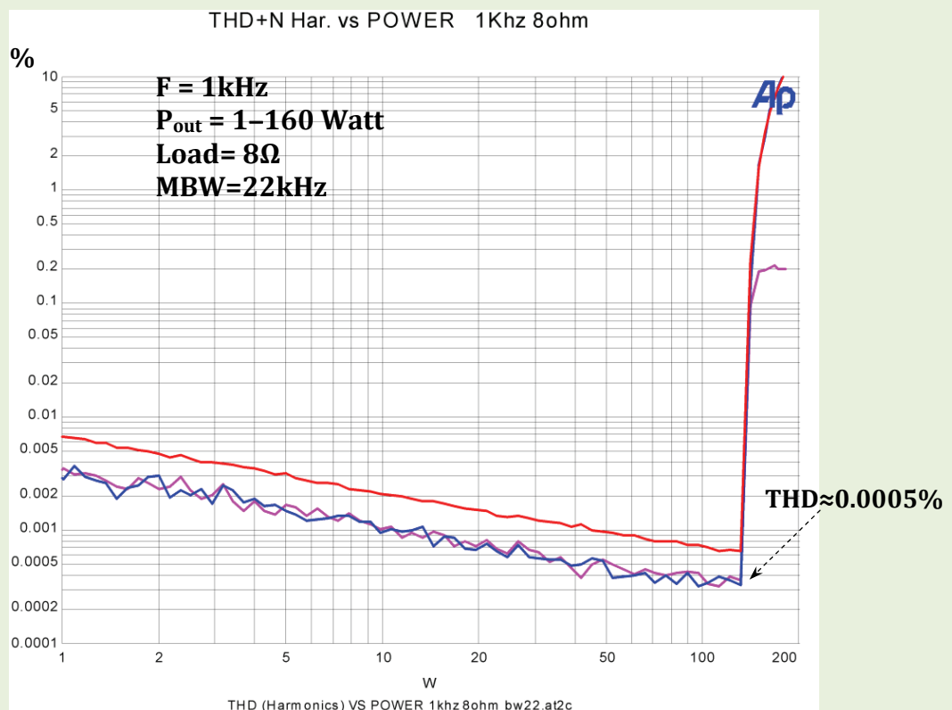
Fig. 1a: THD+N (%) versus power. Frequency = 1kHz, Load = 8 Ω. Measurement bandwidth (MBW) = 22kHz
