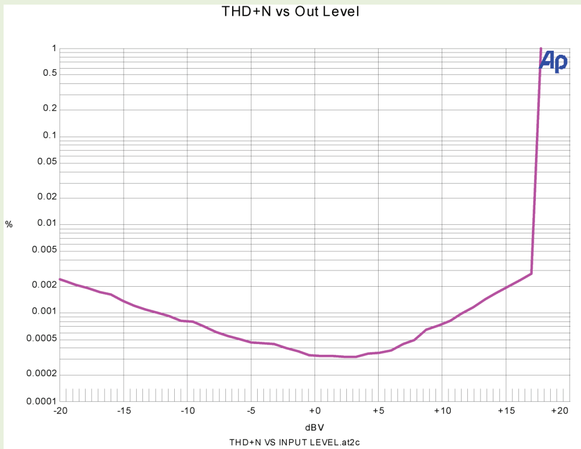
Fig. 2: THD+N (%) versus output level. Freq=1kHz. THD+N at nominal output voltage (0dBV)= 0.0003%
