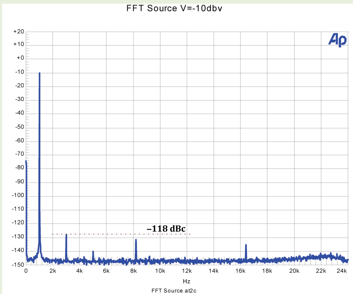
Fig. 3a: DC-24 kHz harmonic distortion spectrum. Freq=1kHz. Source signal at -10dBV
