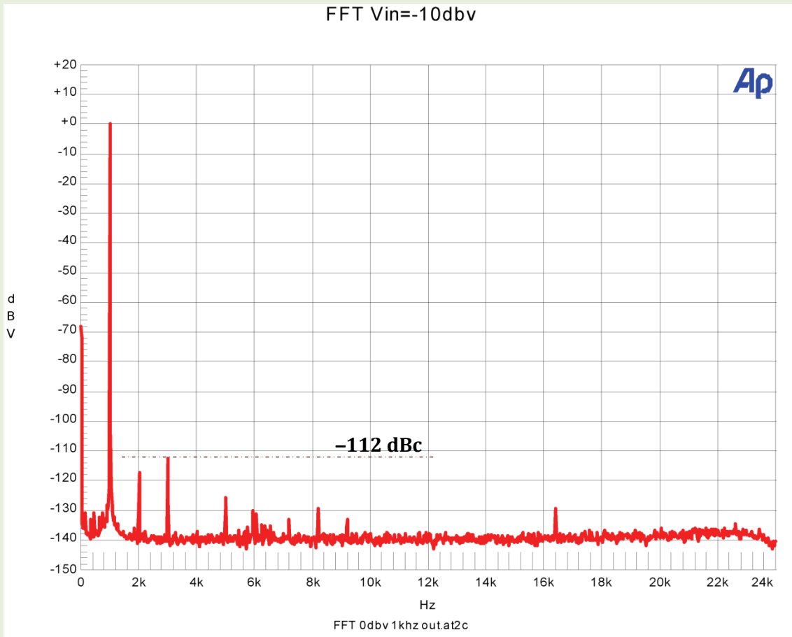
Fig. 3b: DC-24 kHz harmonic distortion spectrum. Freq=1kHz. Output voltage at 0dBV. Volume = 0dB
