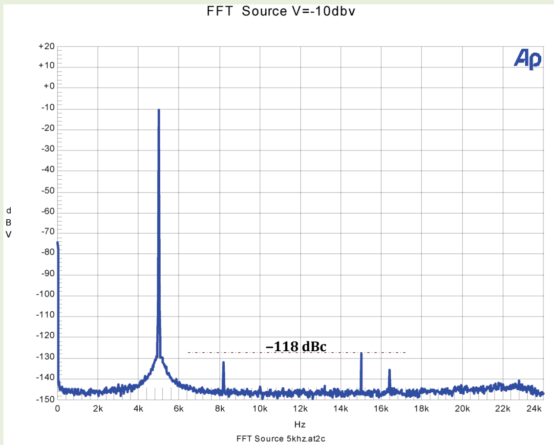
Fig. 4a: DC-24 kHz harmonic distortion spectrum. Freq=5kHz. Source signal at -10dBV
