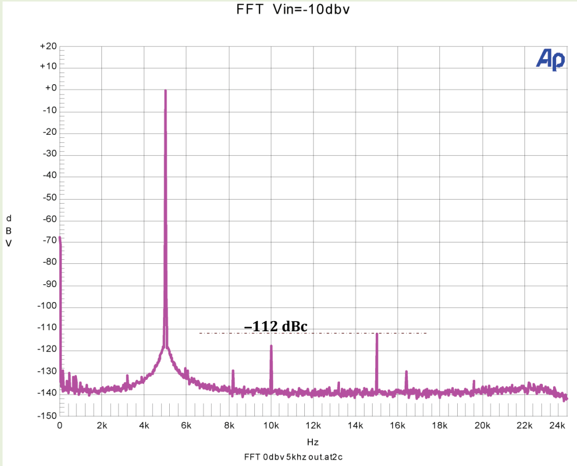
Fig. 4b: DC-24 kHz harmonic distortion spectrum. Freq=5kHz. Output voltage at 0dBV. Volume = 0dB
