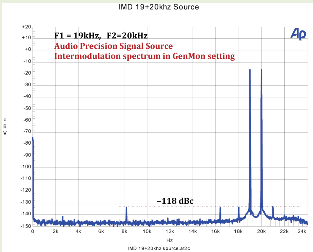
Fig. 5a: DC-24 kHz Intermodulation Distortion spectrum. Freq=19kHz+20kHz. Signal Source with AP test equipment in GenMon setting.
