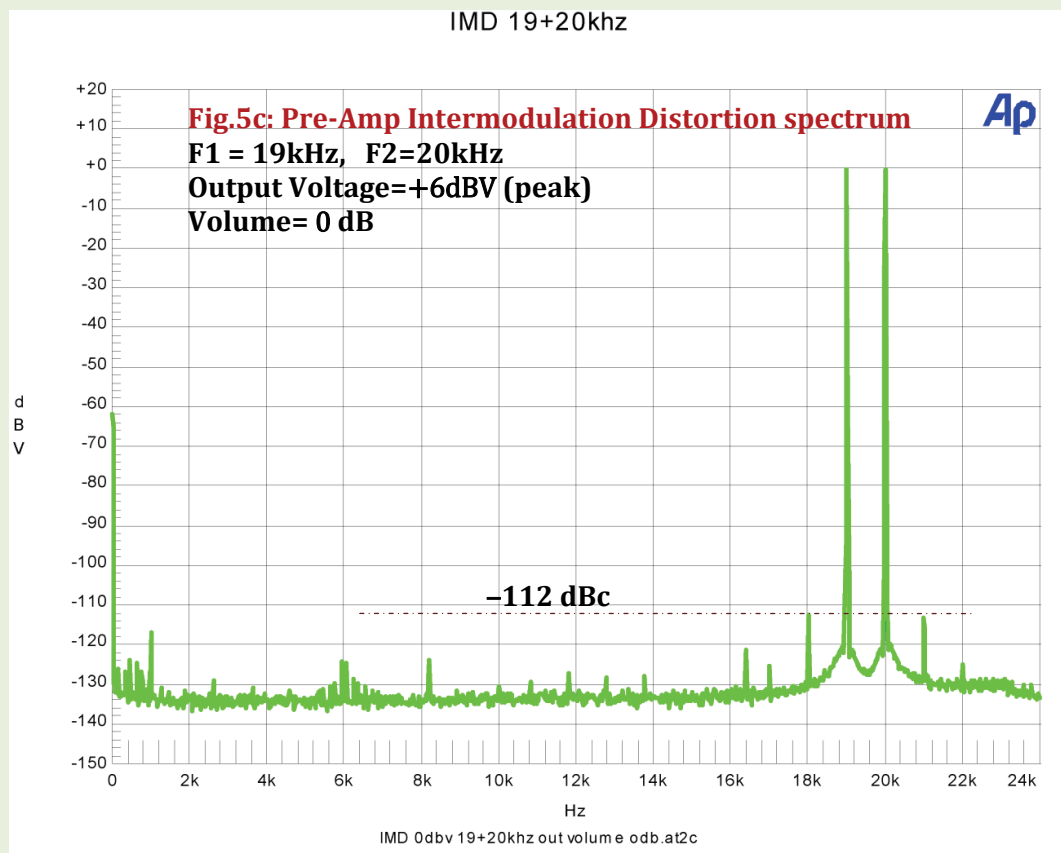
Fig. 5b-5c: DC-24 kHz Intermodulation Distortion spectrum. Freq=19kHz+20kHz.
