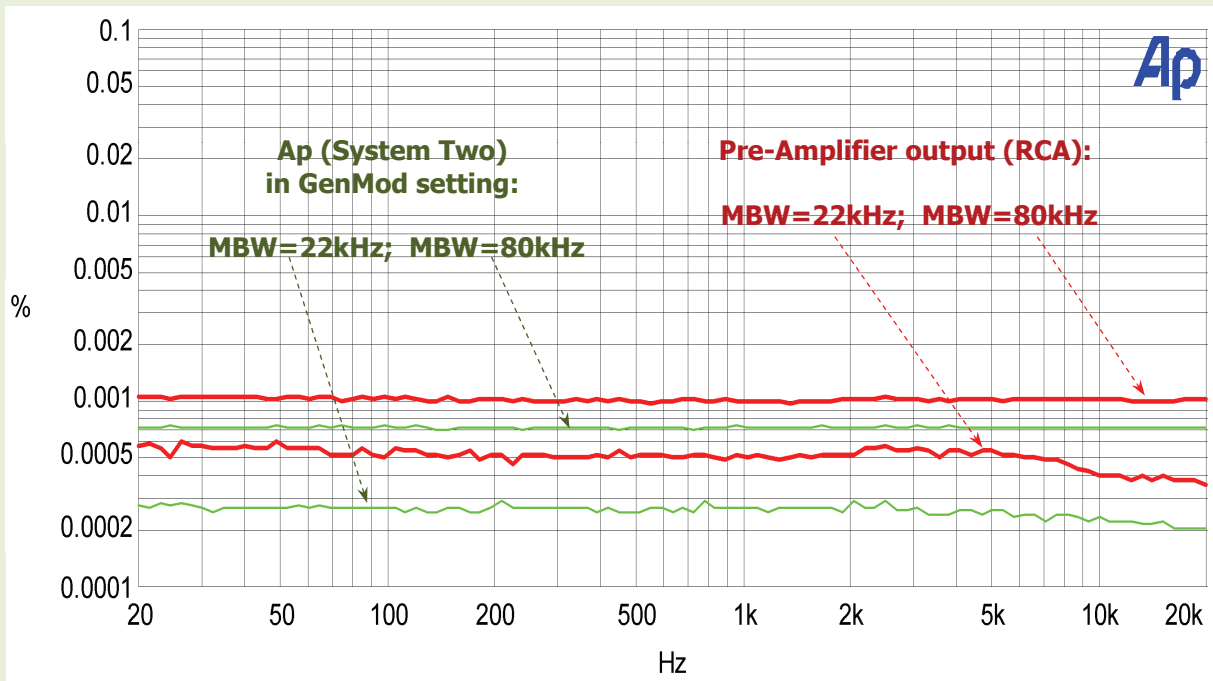
Fig. 2: THD+N (%) versus frequency: Freq=20 Hz – 20kHz. Input level: 500mV. Output level: 0dBV; Volume: 0dB (max)
